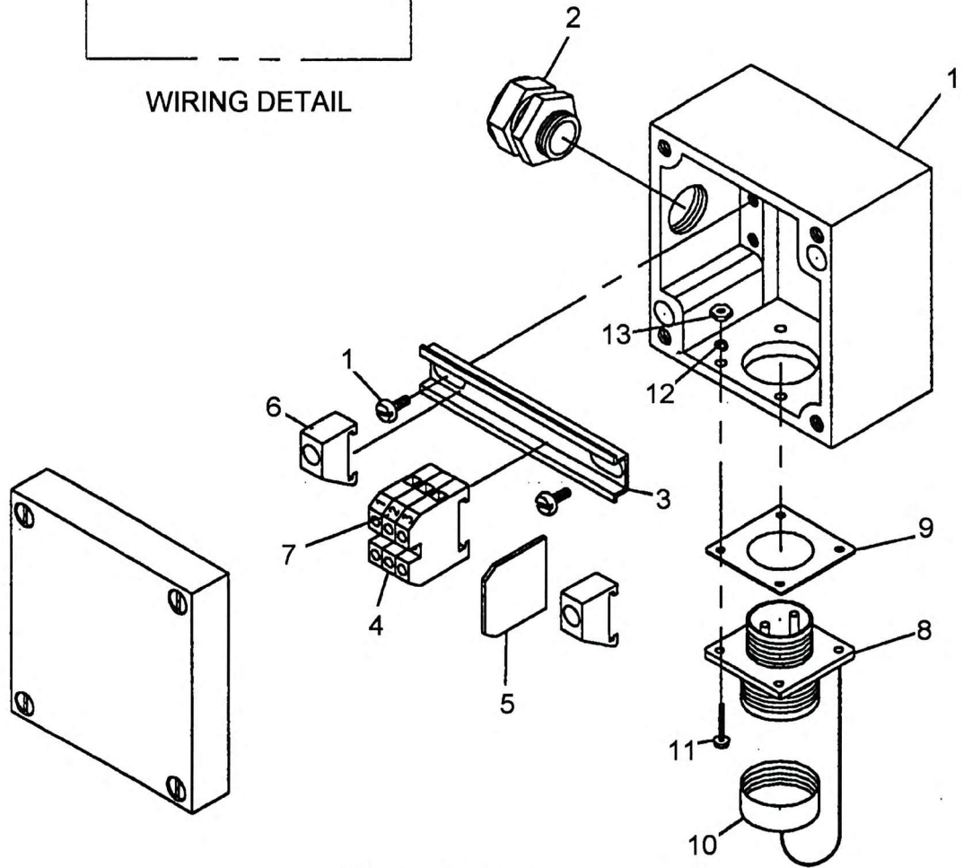
EXPLODED VIEW
